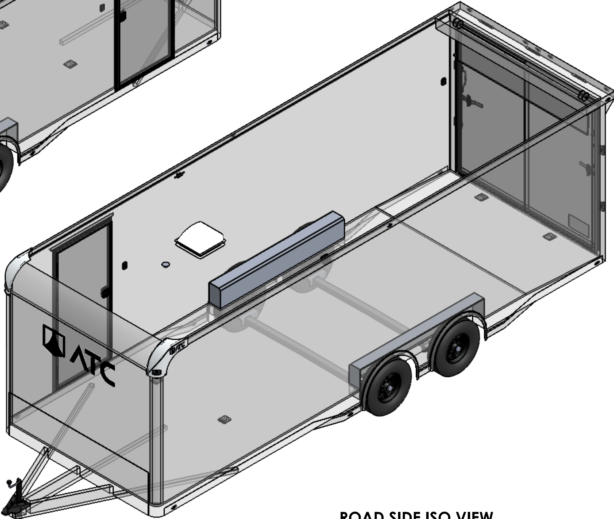
ROAD SIDE ISO VIEW
