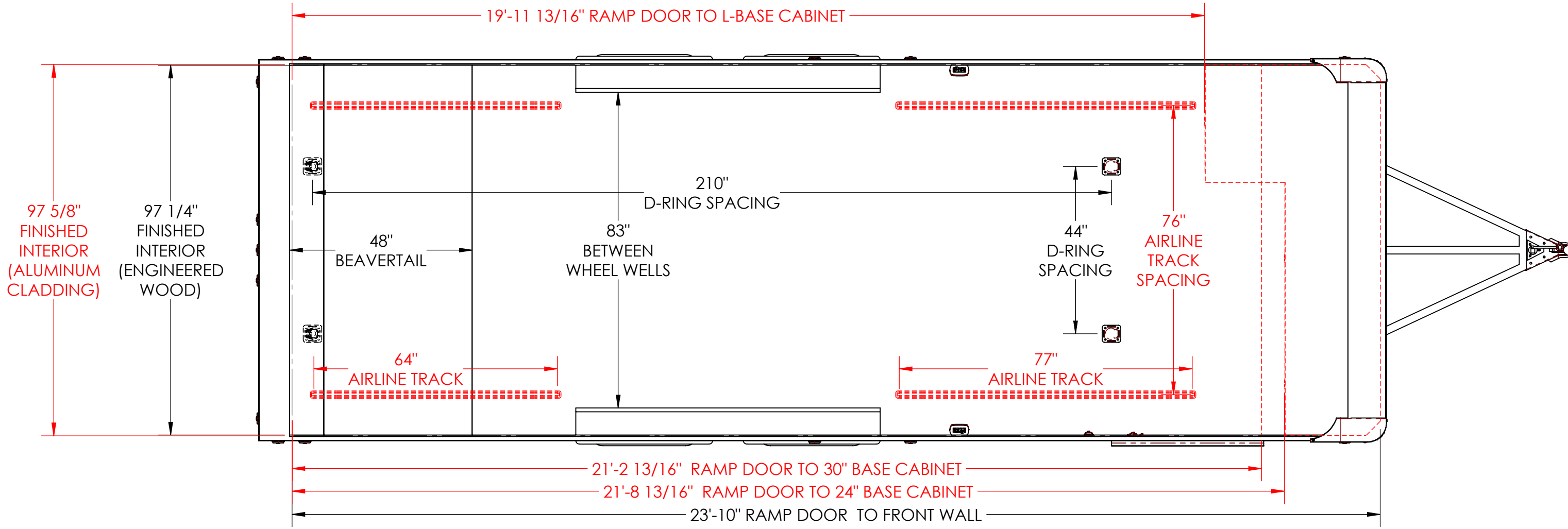
TOP VIEW FLOORPLAN LAYOUT
