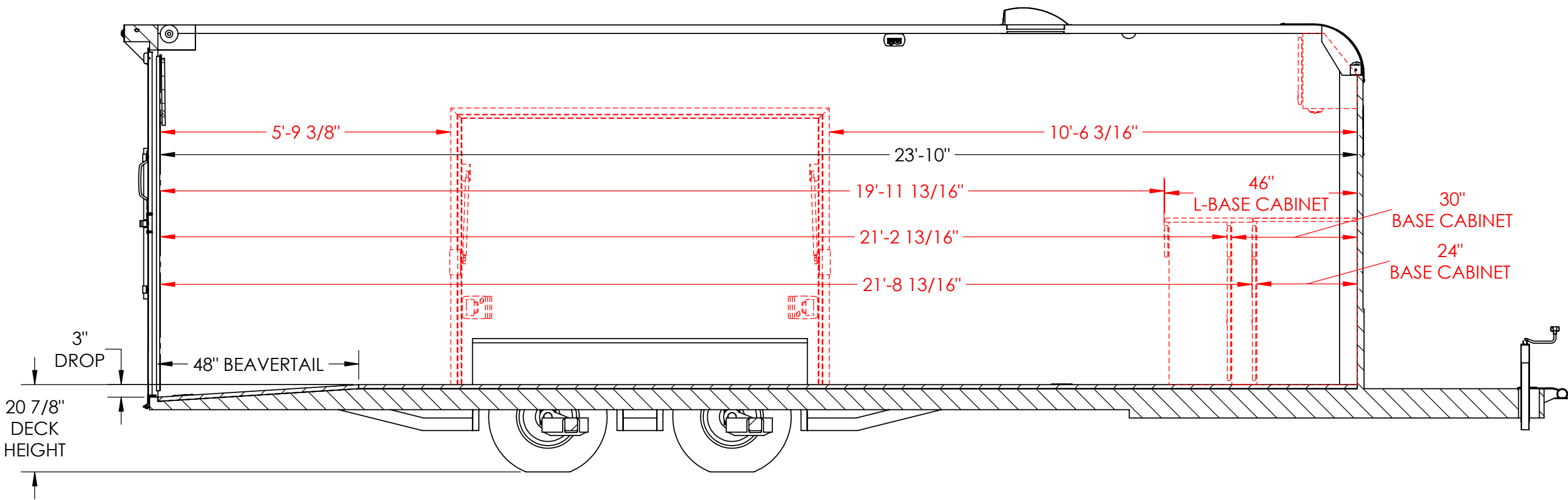
INTERIOR ROAD SIDE SECTION A-A
