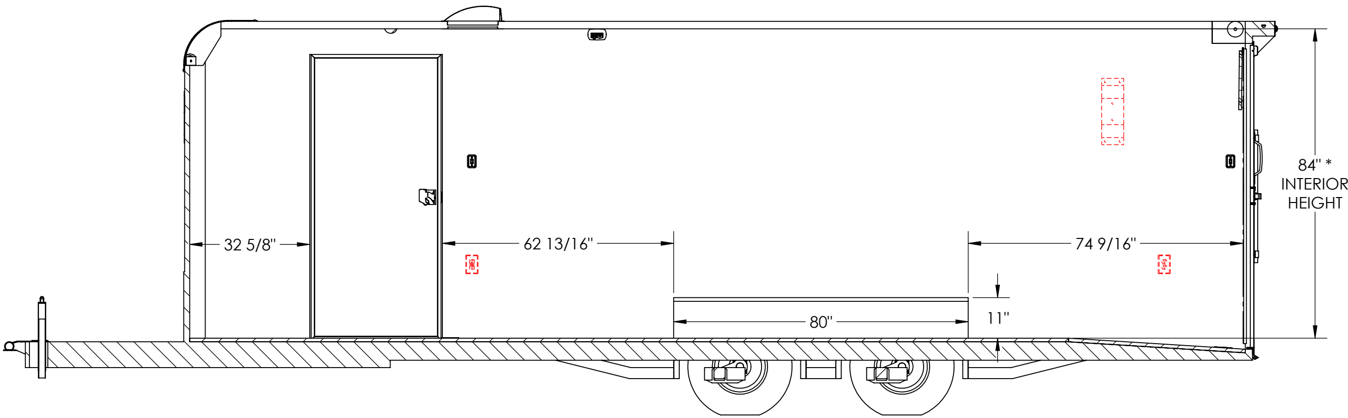
INTERIOR CURB SIDE SECTION B-B
